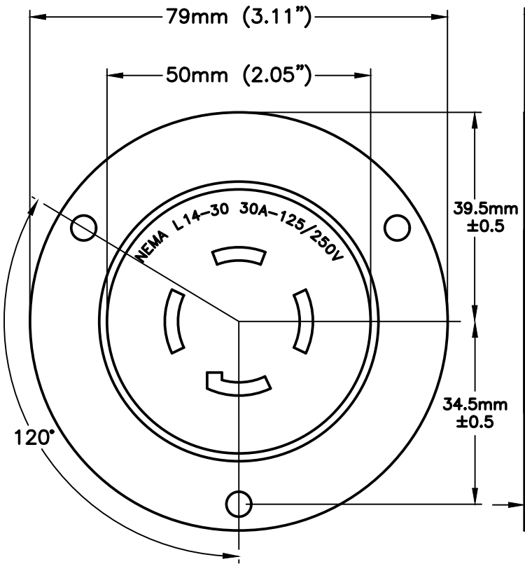
NEMA L14-30 RECEPTACLE FRONT VIEW
